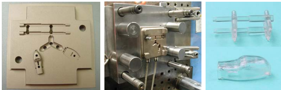
Figure 1: Series production of an LED light guide in polycarbonate.
